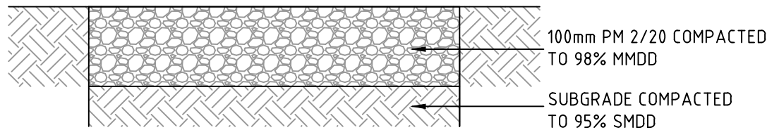
TYPICAL FOOTPATH CROSS SECTION NOT TO SCALE
