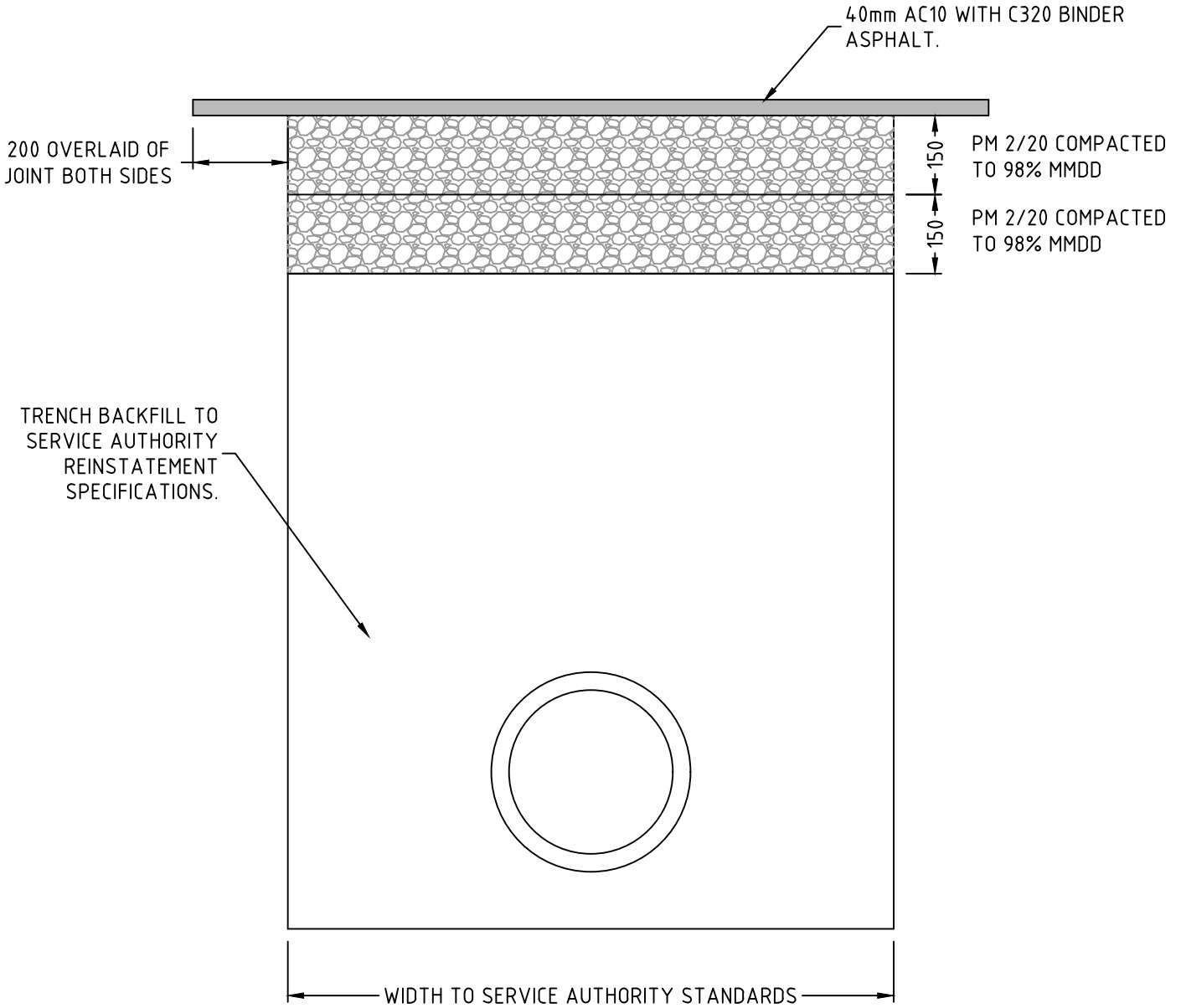
TRENCH REINSTATEMENT NOT TO SCALE
